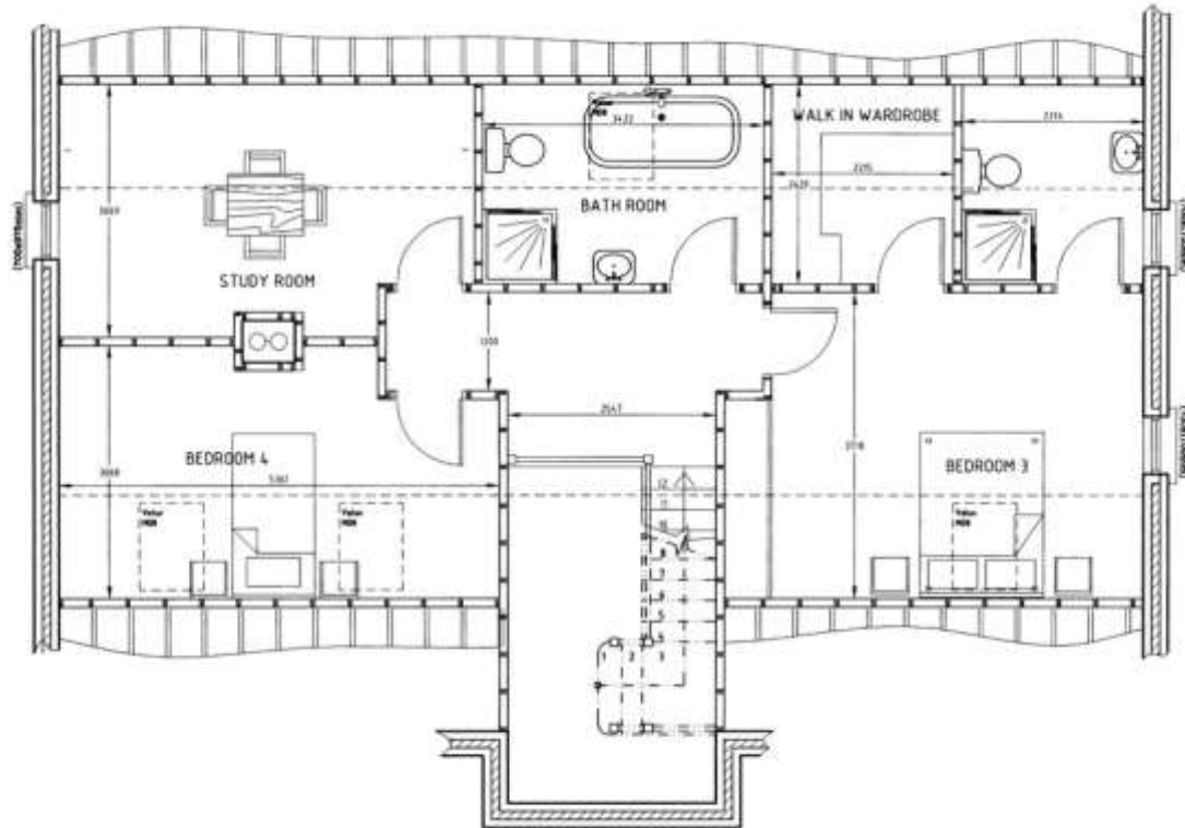
UPSTAIRS LAYOUT PLAN
