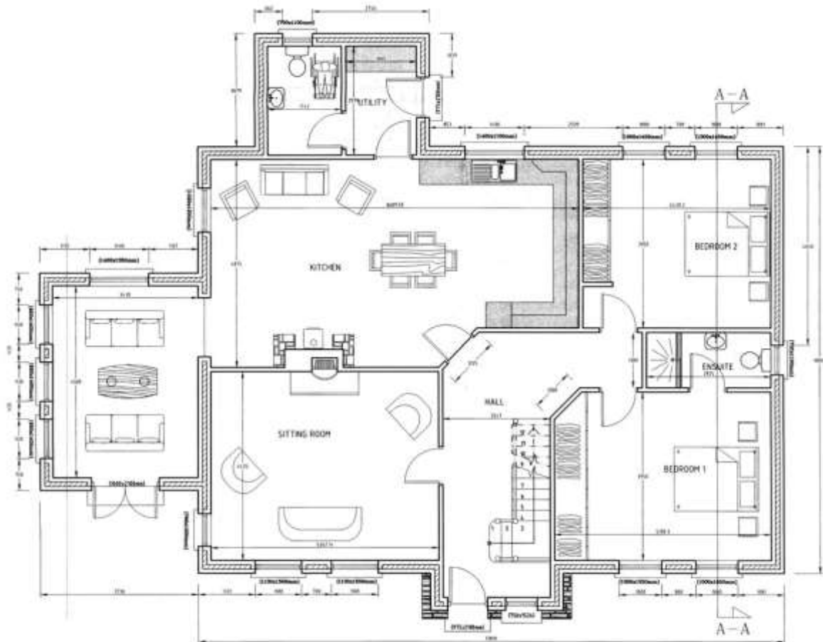
GROUND FLOOR LAYOUT PLAN Ground Floor Plans of Proposed House
