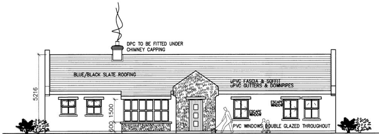
FRONT ELEVATION 1:100
