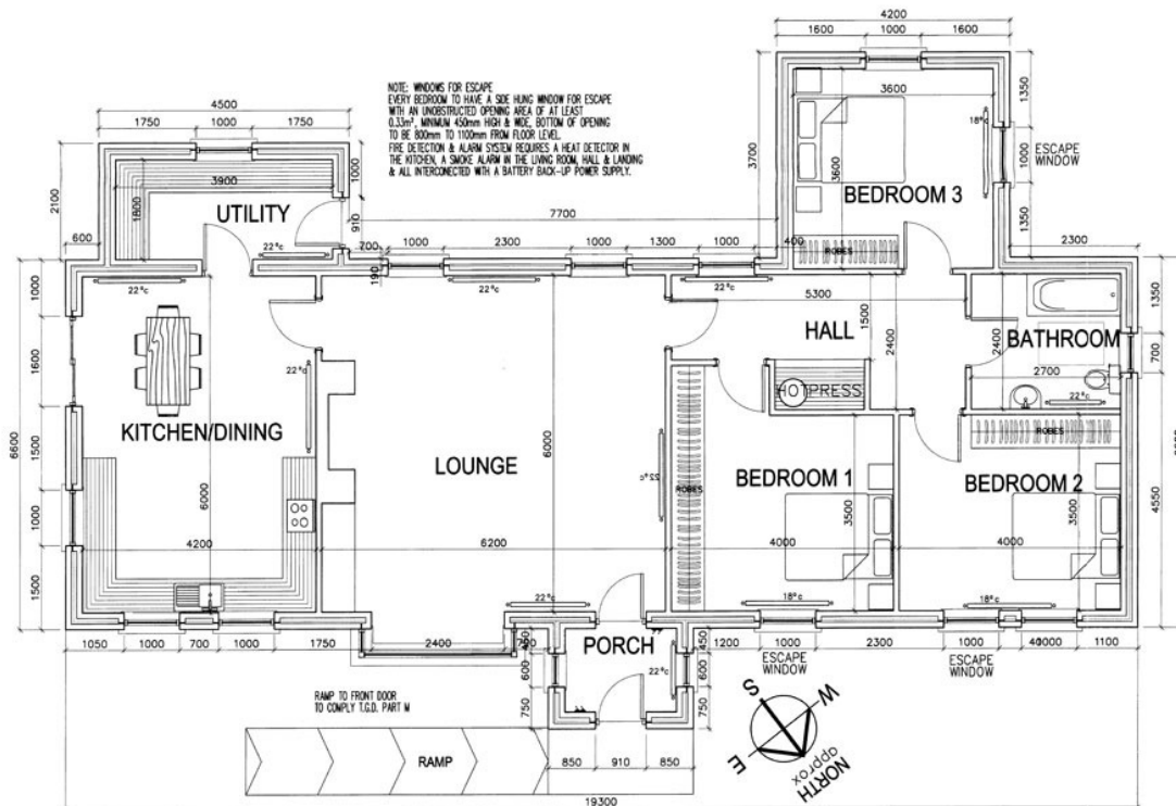
FLOOR PLAN 1:50 FLOOR AREA = 138.90 SQ M
