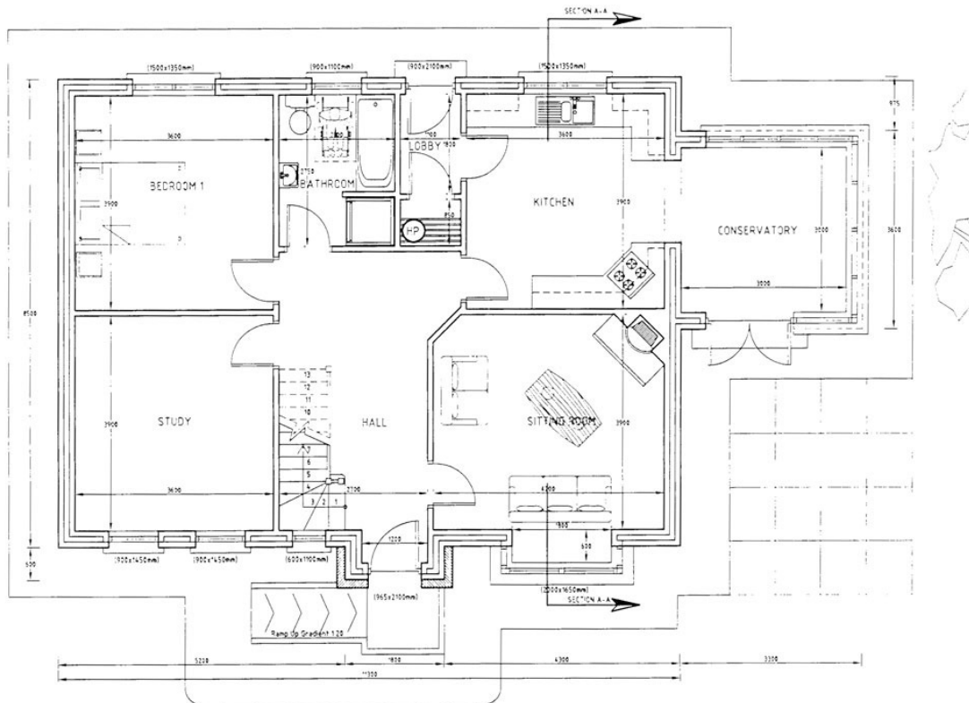
GROUND FLOOR LAYOUT PLAN
