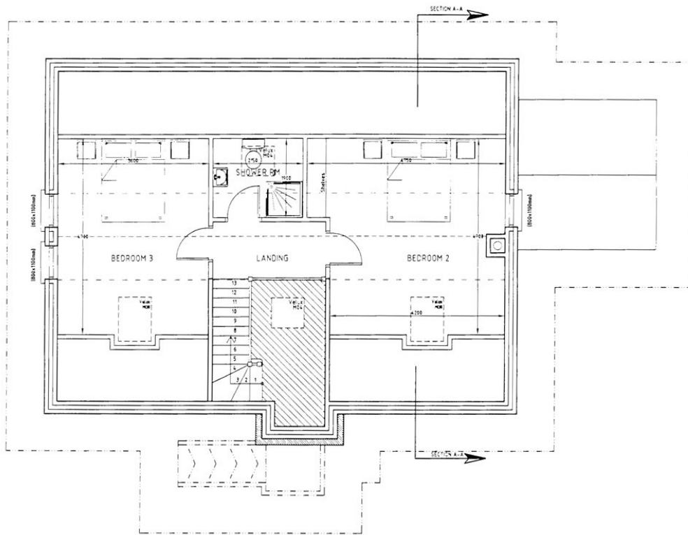
UPPER FLOOR LAYOUT PLAN
