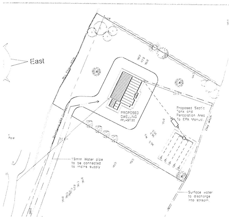
Site Layout
